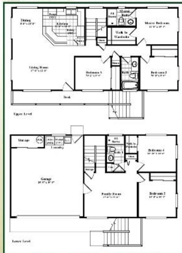
OVERALL DIMENSIONS 32' x 48' ENHANCED FLOOR PLAN
